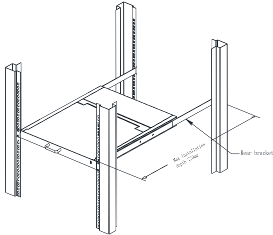
1-2.2 rack mounting (2)
