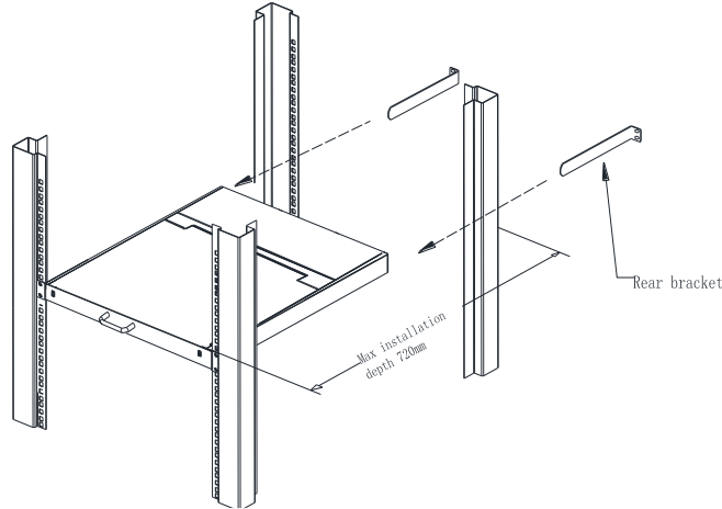
1-2.1 rack mounting (1)
