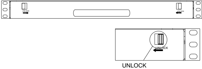
2-1.3 unlocking
