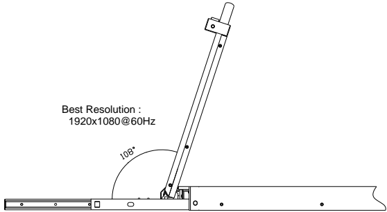
2-1.4 rotate angle of the console
